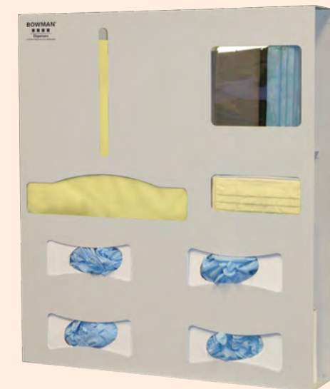
PS412-0512 Holds gowns, aprons, overalls/ jumpsuits, gloves, masks and shields Size: W-22.75"xH-25.63"xD-4"
